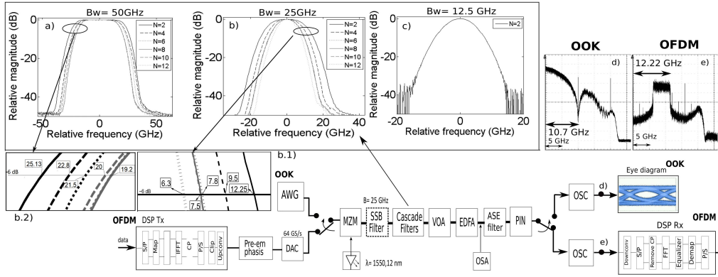
Fig. 2. Experimental setup for OOK and DD OFDM approach. Cascade filters characterized by the OSA for nominal bandwidths of 50 GHz a), 25 GHz b) and 12.5 GHz c). Received spectra after the oscilloscope for OOK d) and OFDM e) alternatives.
