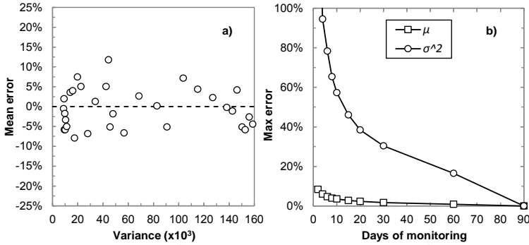
Fig. 6. Mean error of \sigma^2 estimation (a) and max. error of \mu and \sigma^2 vs. days of monitoring (b).
