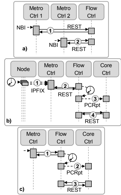
Fig. 4. Metro-flow set-up (a), Metro-flow model estimation (b) and Metro-flow rerouting (c).
