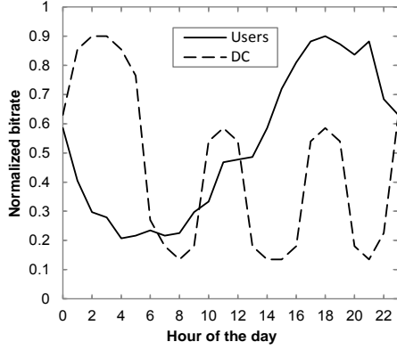
Fig. 5. Users and DC metro-flow traffic profiles.
