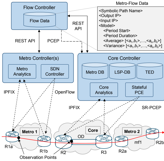
Fig. 3. Proposed network architecture.
