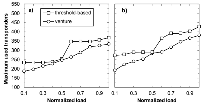
Fig. 9. Maximum used transponders under randomized (a) and per type of service (b) rerouting schemes.
