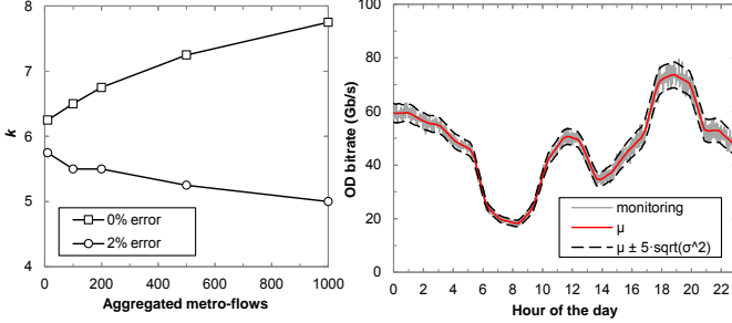
Fig. 8. (a) Value of k (eq. (8)) vs. number of aggregated metro-flows and (b) Prediction of min/max/avg OD bitrate during one day.
