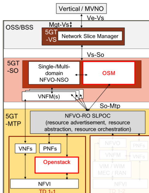
Figure 28: 5G-TRANSFORMER MANO-centric
