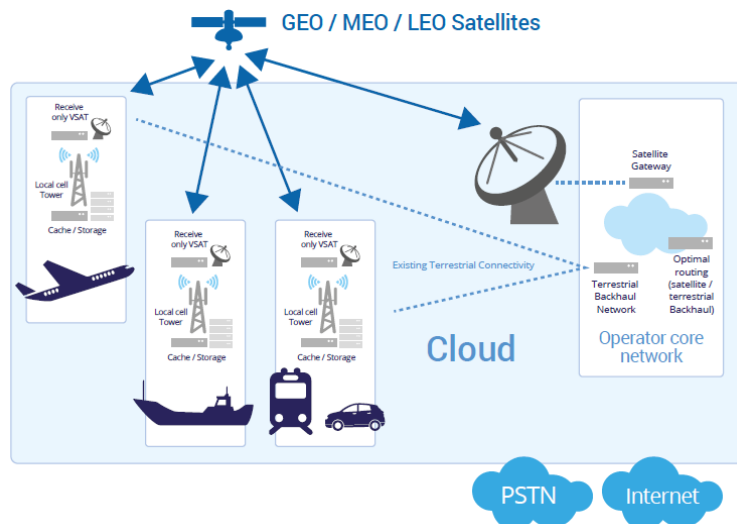
Figure 31: 5G connectivity services to passengers
